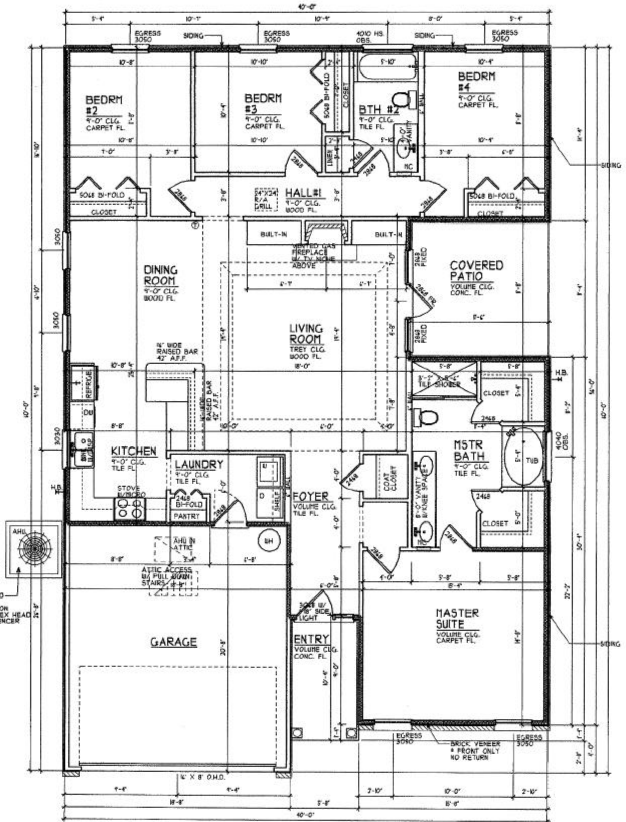
FLOOR PLAN SCALE: 1/4"=1'-0" SCALE: 1/8"=1'-0" (50% REDUCED SET)
