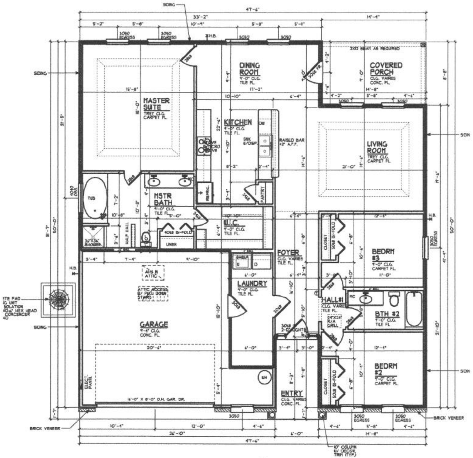
FLOOR PLAN SCALE: 1/8"=1'-0" SCALE: 1/8"=1'-0" (# 50A REDUCED SET)
